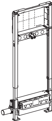
Art. no. 111.580.00.1 floor construction height from 90 mm
