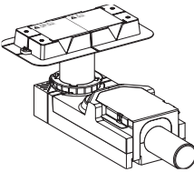
Art. no. 154.150.00.1 floor construction height from 90 mm
